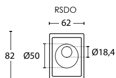
RSDO ΕΠΙΣΤΟΜΙΟ defender ESCUTHEON defender
